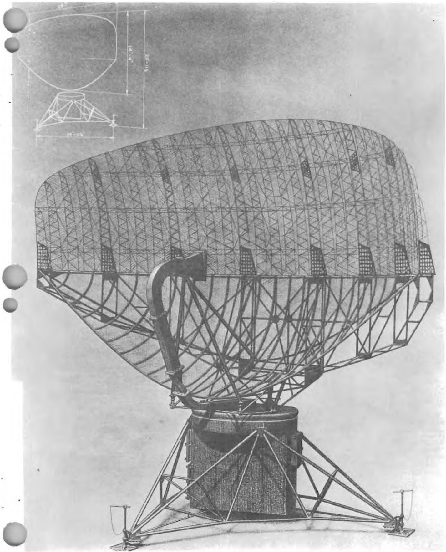
AN/CPS-5
