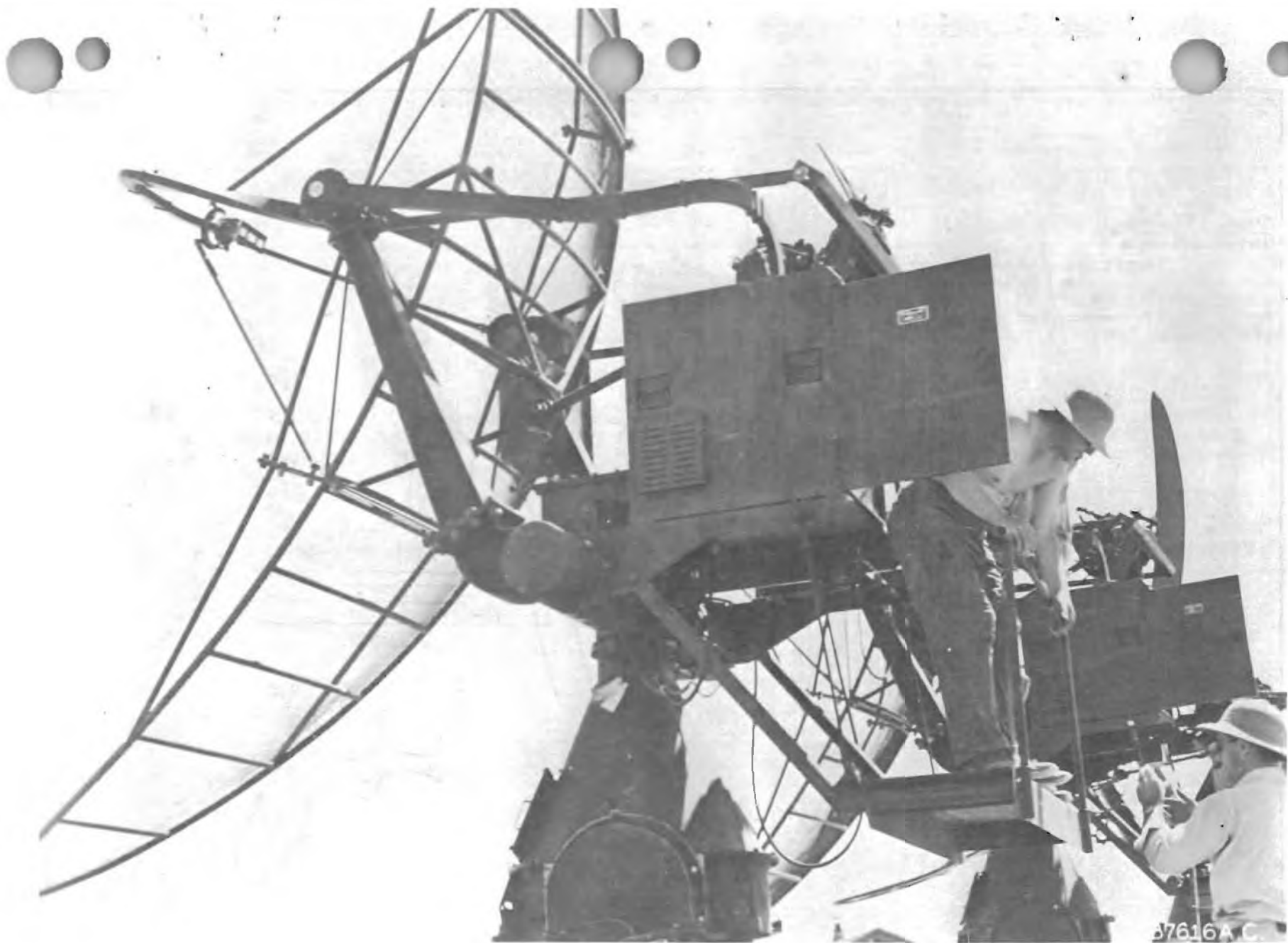
GCI- AN/CPS-4 Height Finder
