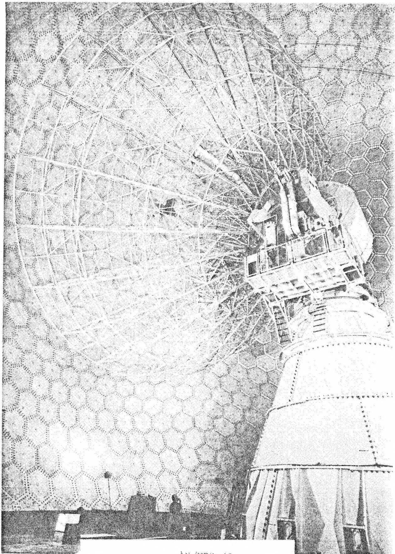
AN/FPS-49 Moorestown
