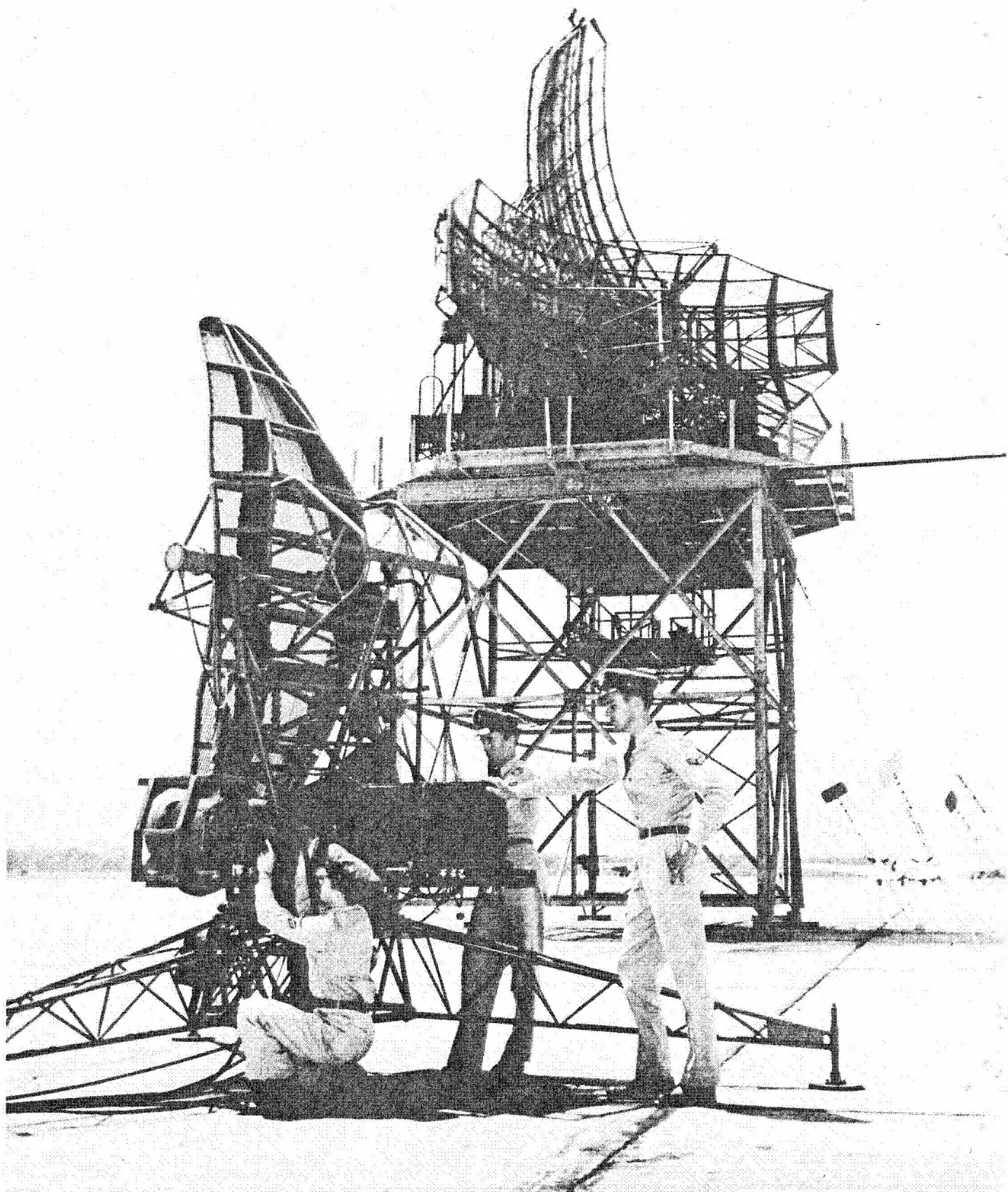
GCI - AN/TPS-10D Height Finder radar in foreground. AN/CPS-6 V beam search and height finder radar in background.
