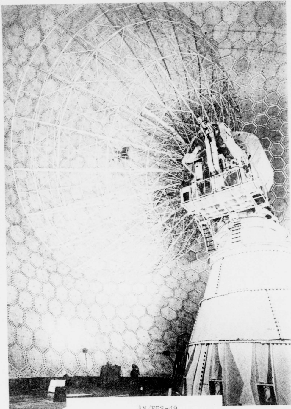
AN/FPS-49 Moorestown
