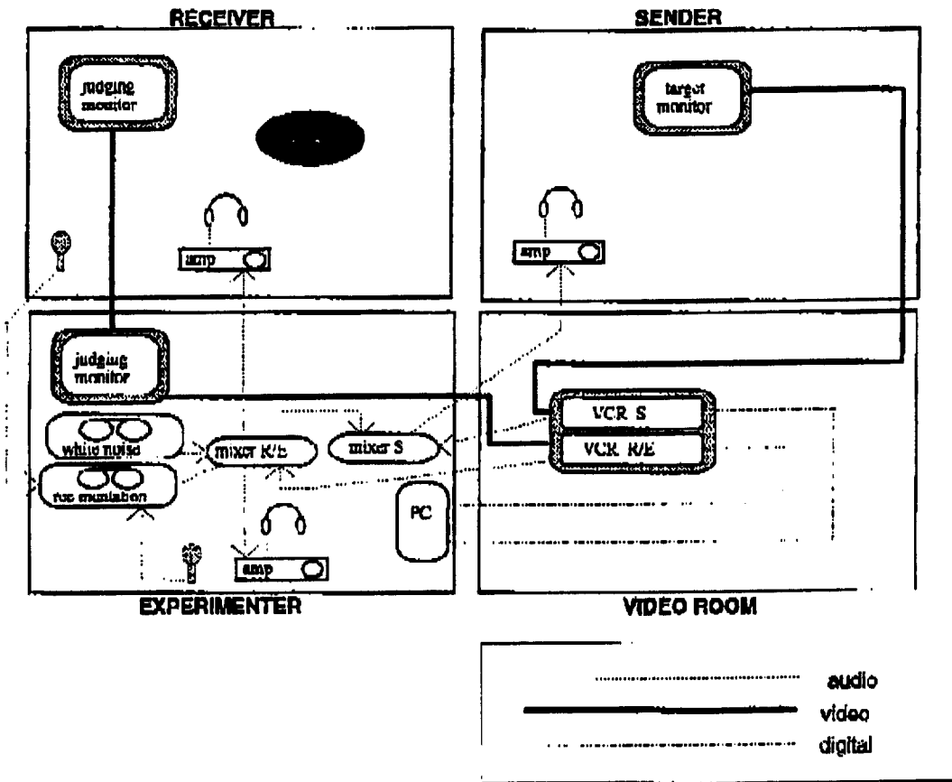
Figure 2. Audio, video, and digital communications layout. This design isolates the audio and video (a/v) paths for S and R/E to avoid introducing sensory cues. The only direct connection between S's and R's a/v systems is the output of the audio mixer into the input of the S audio mixer.
