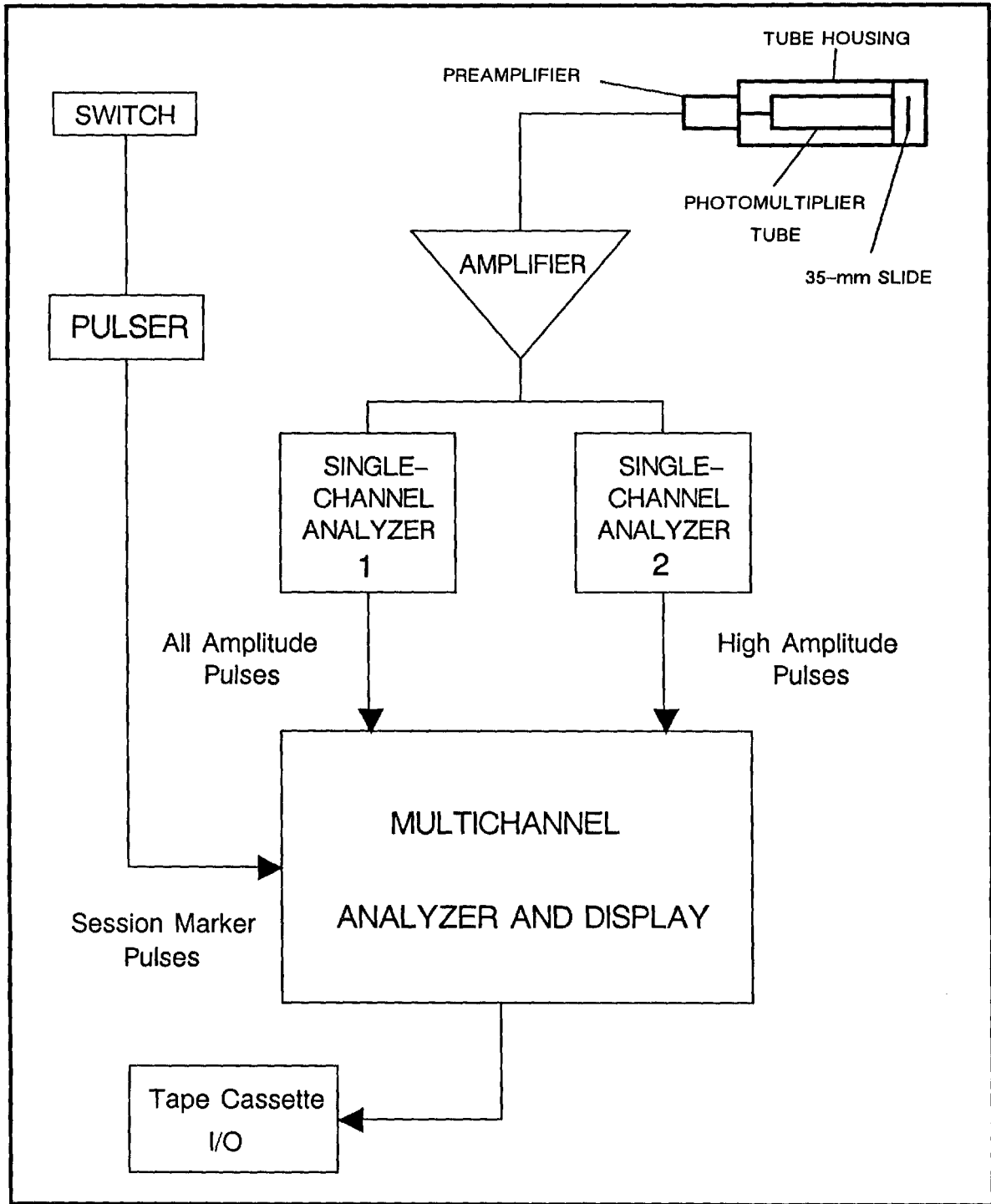
FIGURE 1 (U) SCHEMATIC DIAGRAM FOR THE PHOTON-PRODUCTION EQUIPMENT
