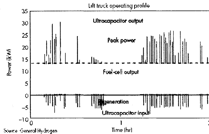
Figure 6. Ultrapacitor Use in a Forklift. Ultracaps provide energy storage upon descent of a load and deliver peak power to lift heavy loads in fuel cell powered forklifts. 23
