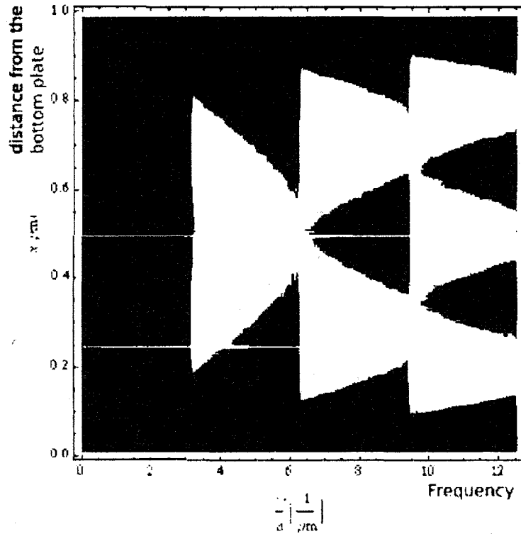
Figure 19. Predicted Casimir Spectral Density \sigma_{yy} (courtesy of P. Marecki) \sigma_{yy} is related to the expected output of a BHD with the LO polarized along the y -direction (parallel to the plates) for the ground state in the Casimir cavity. This is plotted as a function of the position x \in [0, a] between the plates (separation a = 1 \mu\text{m} is assumed) and the frequency \omega \in [0, 4\pi c/a] . Negative values (suppression of fluctuations) are shown in deep purple.
