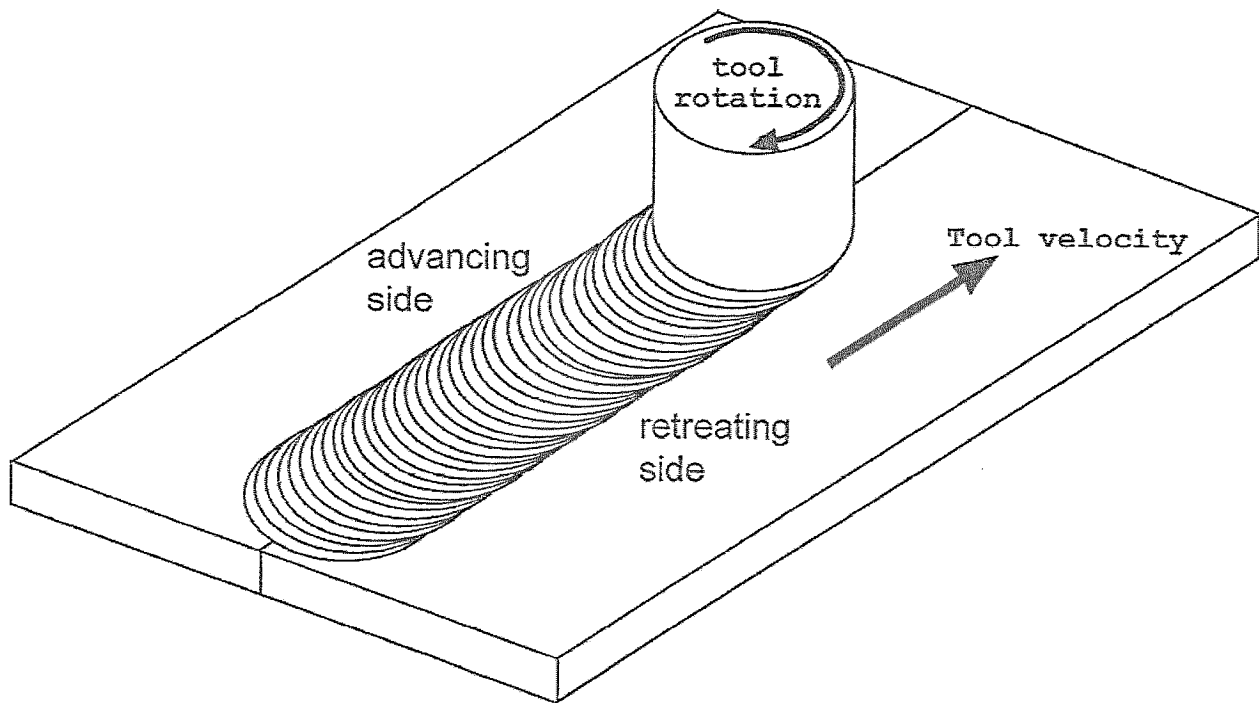
Figure 1. Schematic Diagram of Friction Stir Welding
