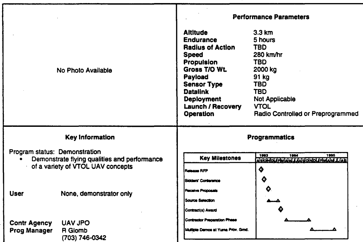
Figure 5-5 Vertical Launch and Recovery
