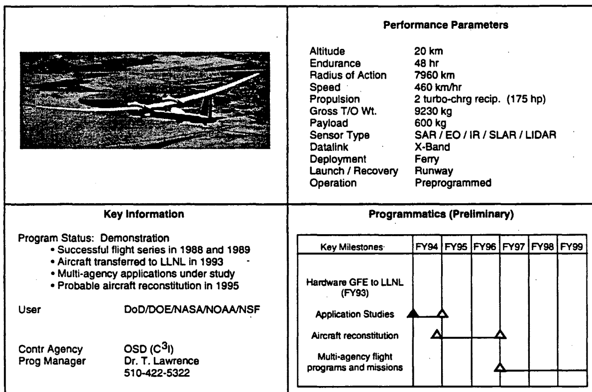
Figure 7-14 Condor High-Altitude, Endurance UAV (Potential Joint Program with Both Defense and Scientific Missions)
