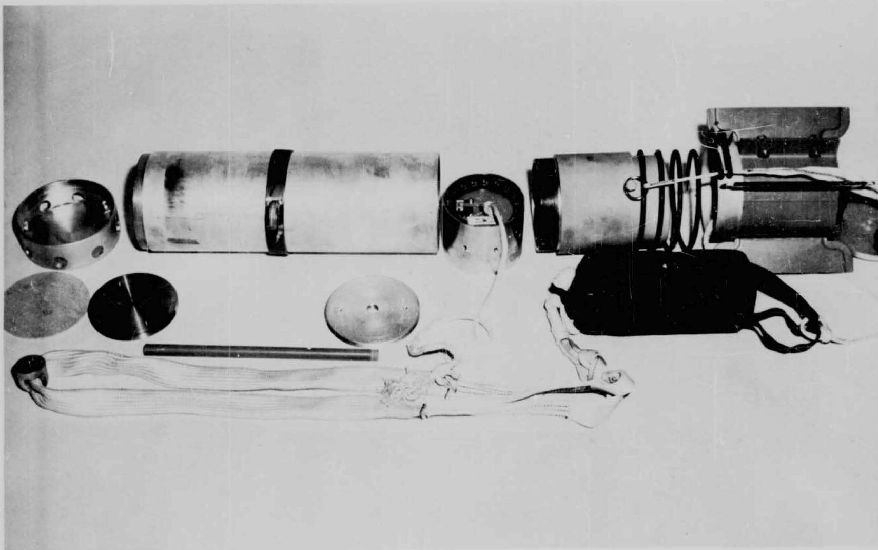
FIG. 4. The Hardware, Parachute, and Fuze Mechanism of the Cyclops Unit.
