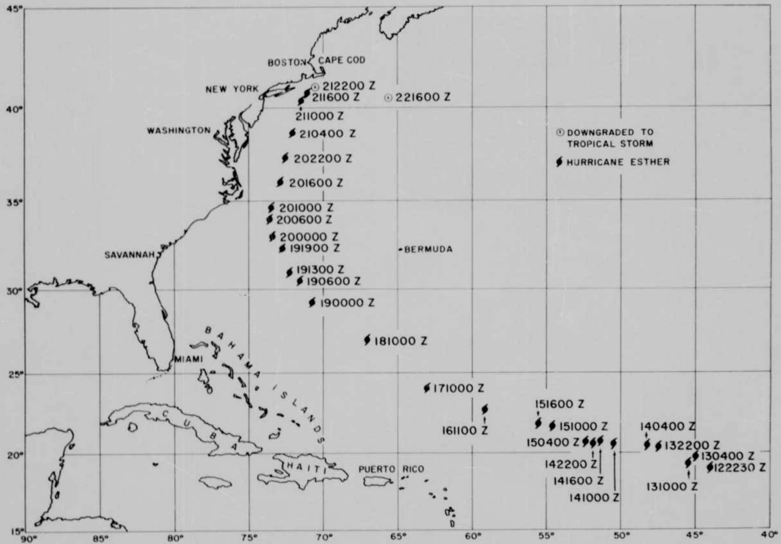
FIG. 22. The Track of Hurricane Esther as Plotted by the Navy Meteorologists at Roosevelt Roads, Puerto Rico.
