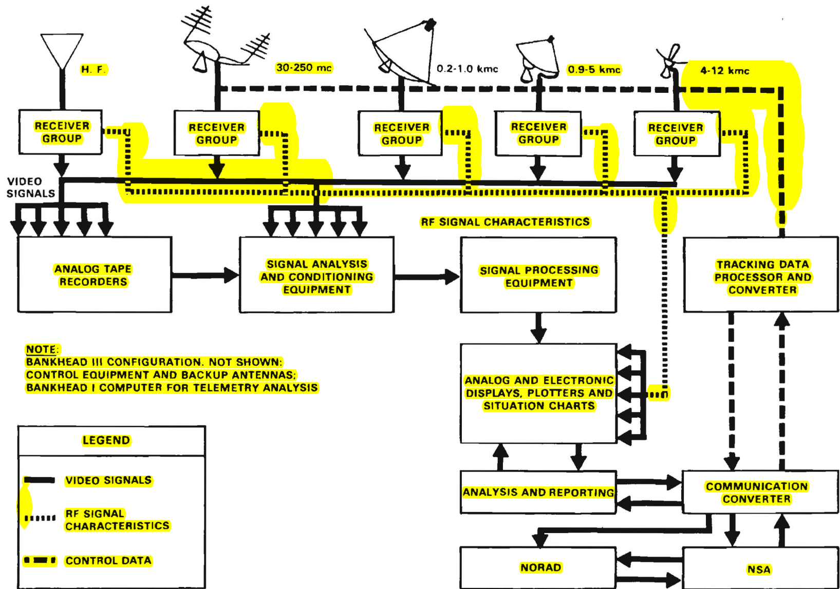
Figure 4 Bankhead System Diagram. (Figure is CONFIDENTIAL.)
